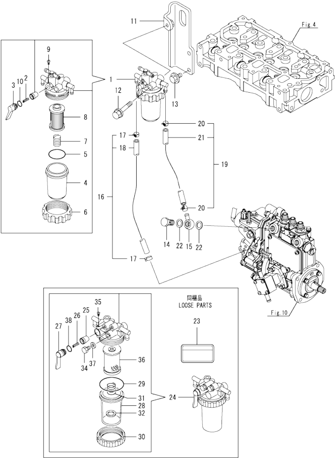
Fig.13. FUEL PIPE
