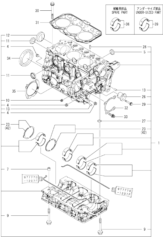
Fig.1. CYLINDER BLOCK
